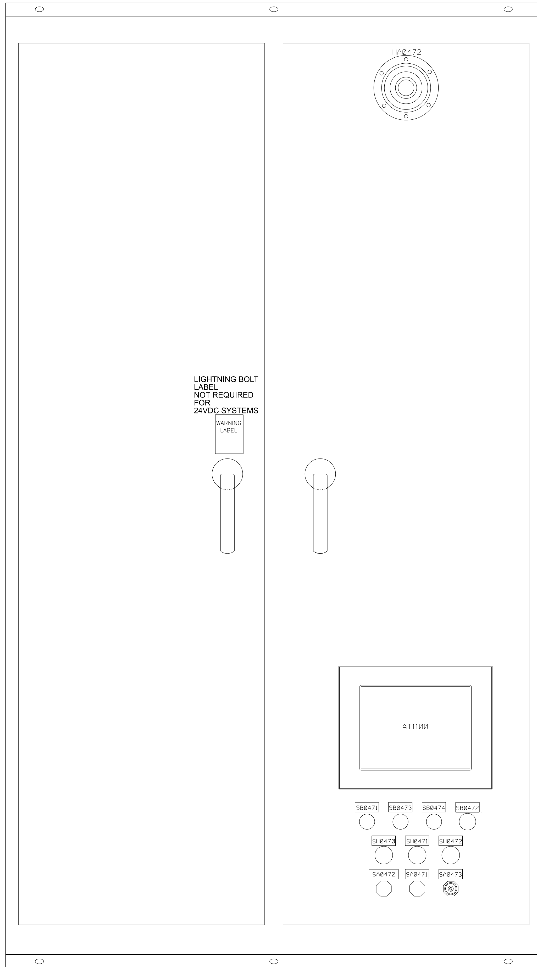
FRONT VIEW
